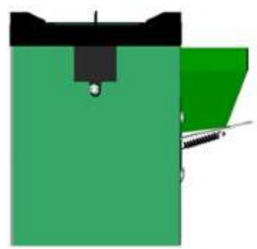
1.4 Left View
