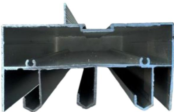
1.2 Front View
