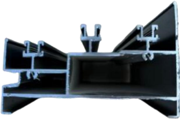
1.2 Front View
