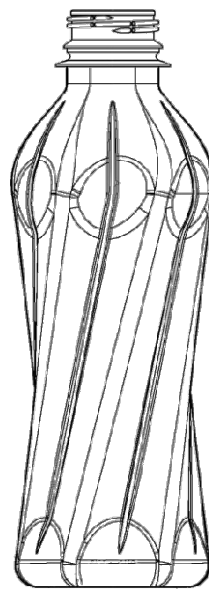
1.4 Left View
